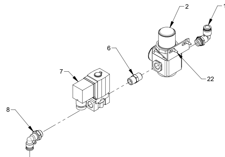
DETAIL A (1 : 4)
