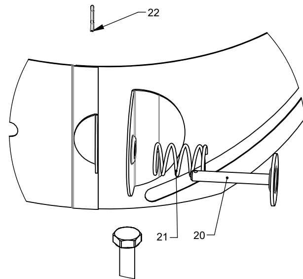
DETAIL B (2 : 5)
