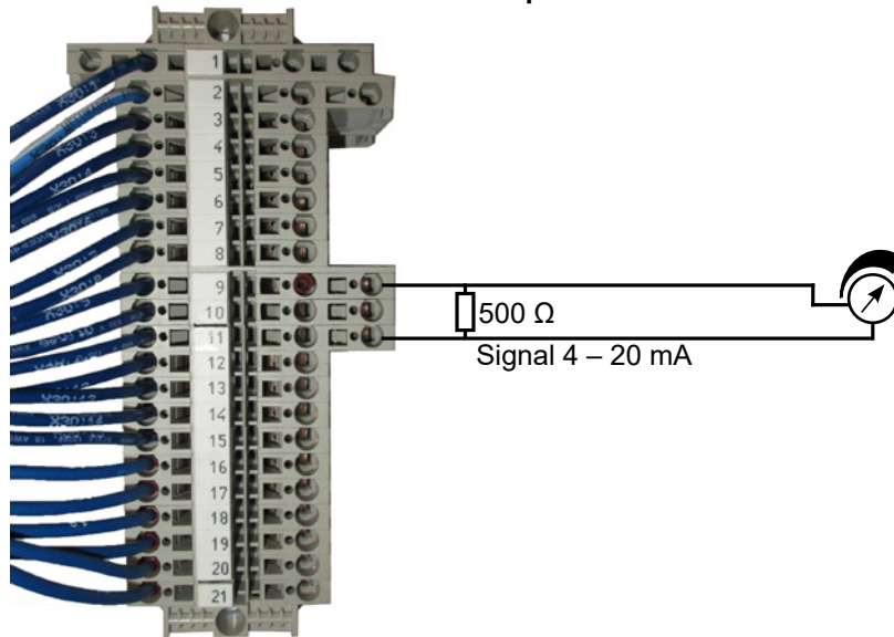
4 – 20 mA setpoint
