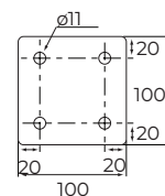
KM 20 – KM 35 Base plate
