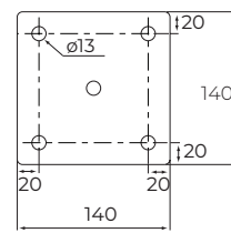
KM 50 – KM 100 Base plate
