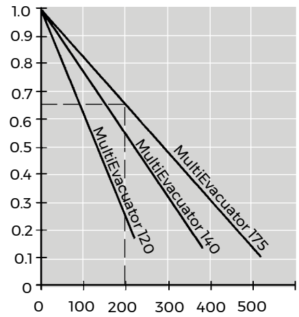
Back pressure [mmWG] (e.g. granulator/shredder)
