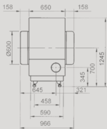
MultiAir 1020T/1040T/1075T uden regulering
