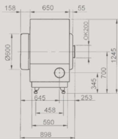
MultiAir 1020S/1040S/1075S uden regulering
