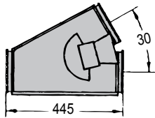
30° 2-way diverter, paint. Pneumatic operated, w/o cylinder. 122 000 697
