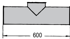
90° branch pipe, paint. OK160/100/160. 122 000 461
