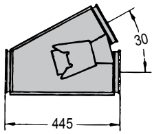
30° 2-way diverter, paint. 122 000 690
