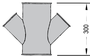
45° OK160 Branch pipe w/2 x OK100 branches, paint. 122 000 805
