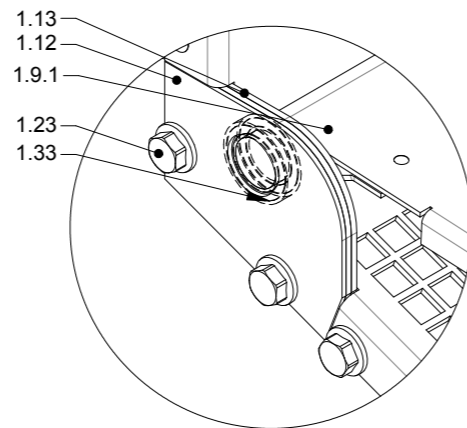
DETAIL G (1 : 2)
