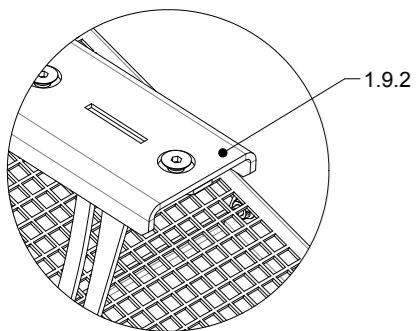
DETAIL E (1 : 4)
