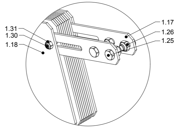
DETAIL C (1 : 4)
