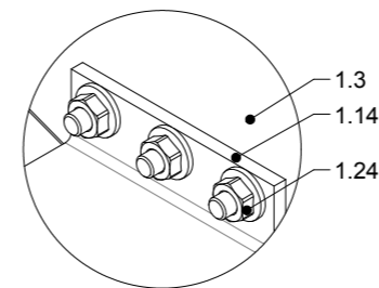
DETAIL H (1 : 2)
