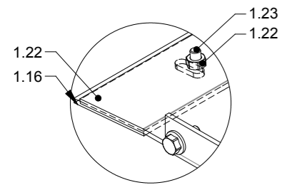
DETAIL A (1 : 3)
