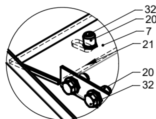
DETAIL A (1 : 3)
