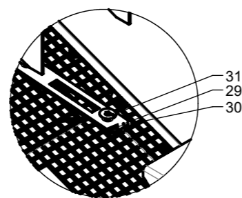
DETAIL G (1 : 5)
