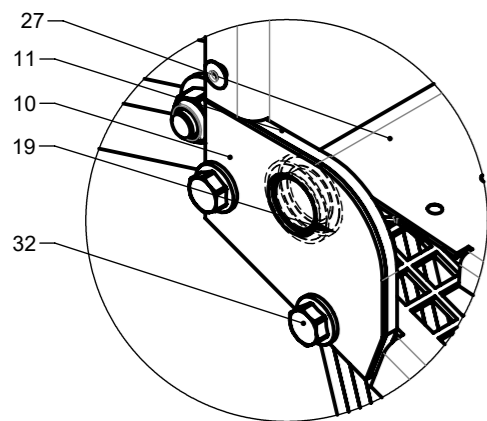
DETAIL E (1 : 2)
