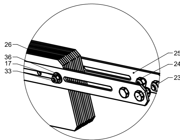
DETAIL C (1 : 4)
