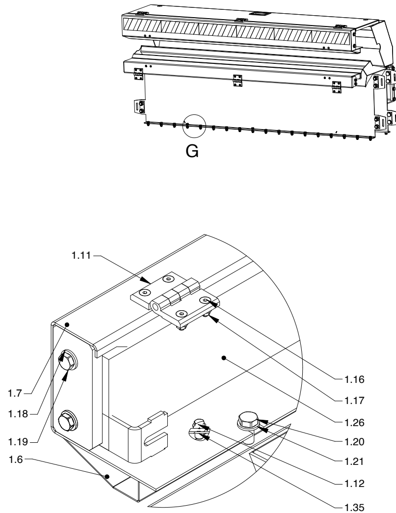
DETAIL E (1 : 4)
