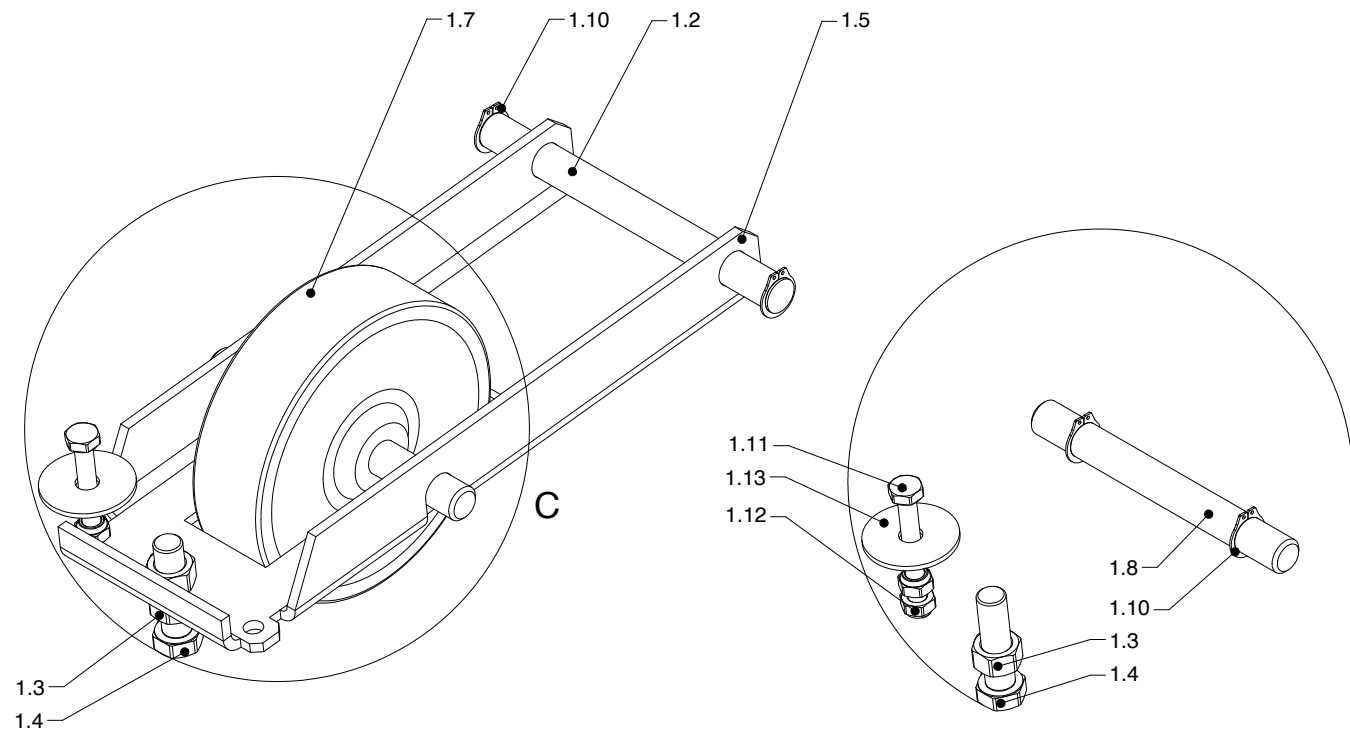
DETAIL A (1 : 4)
