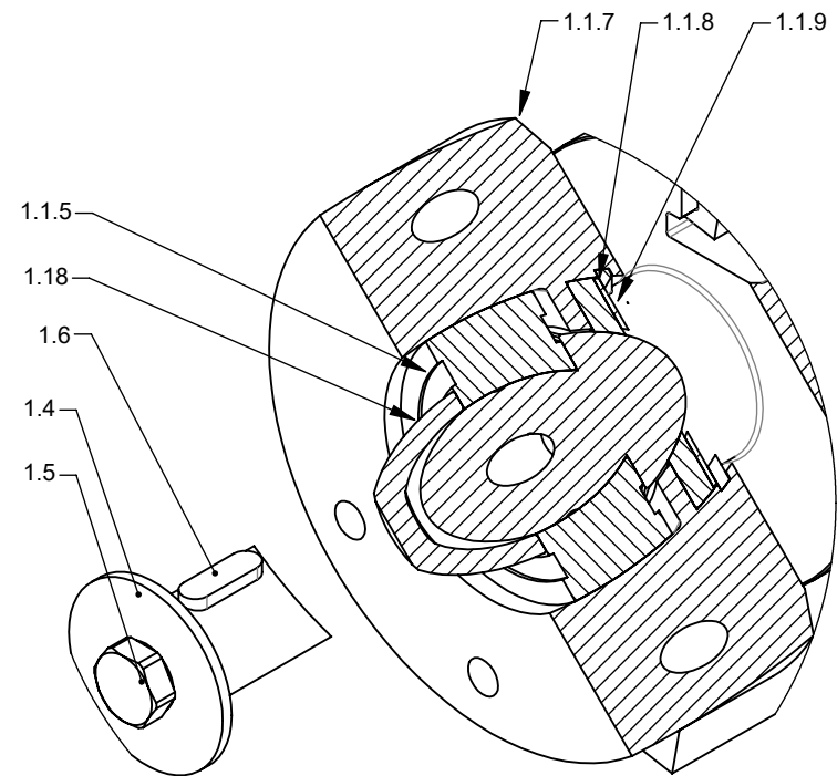
DETAIL A (1 : 2)
