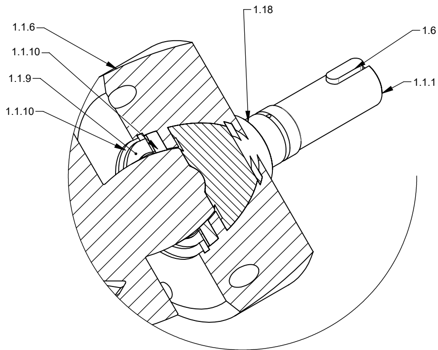
DETAIL C (1 : 2)
