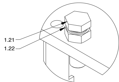
DETAIL A (1 : 3)
