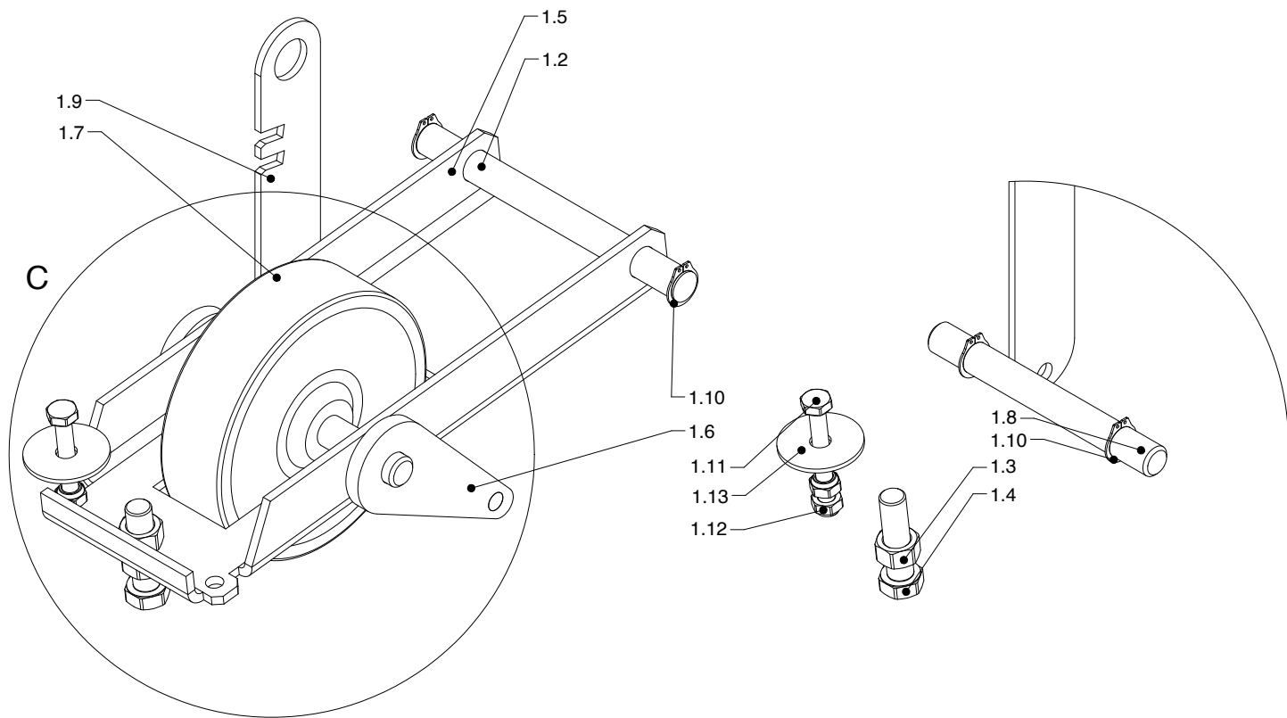
DETAIL C (1 : 4)
