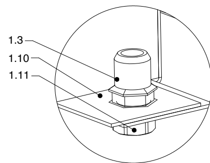
DETAIL B (1 : 1)
