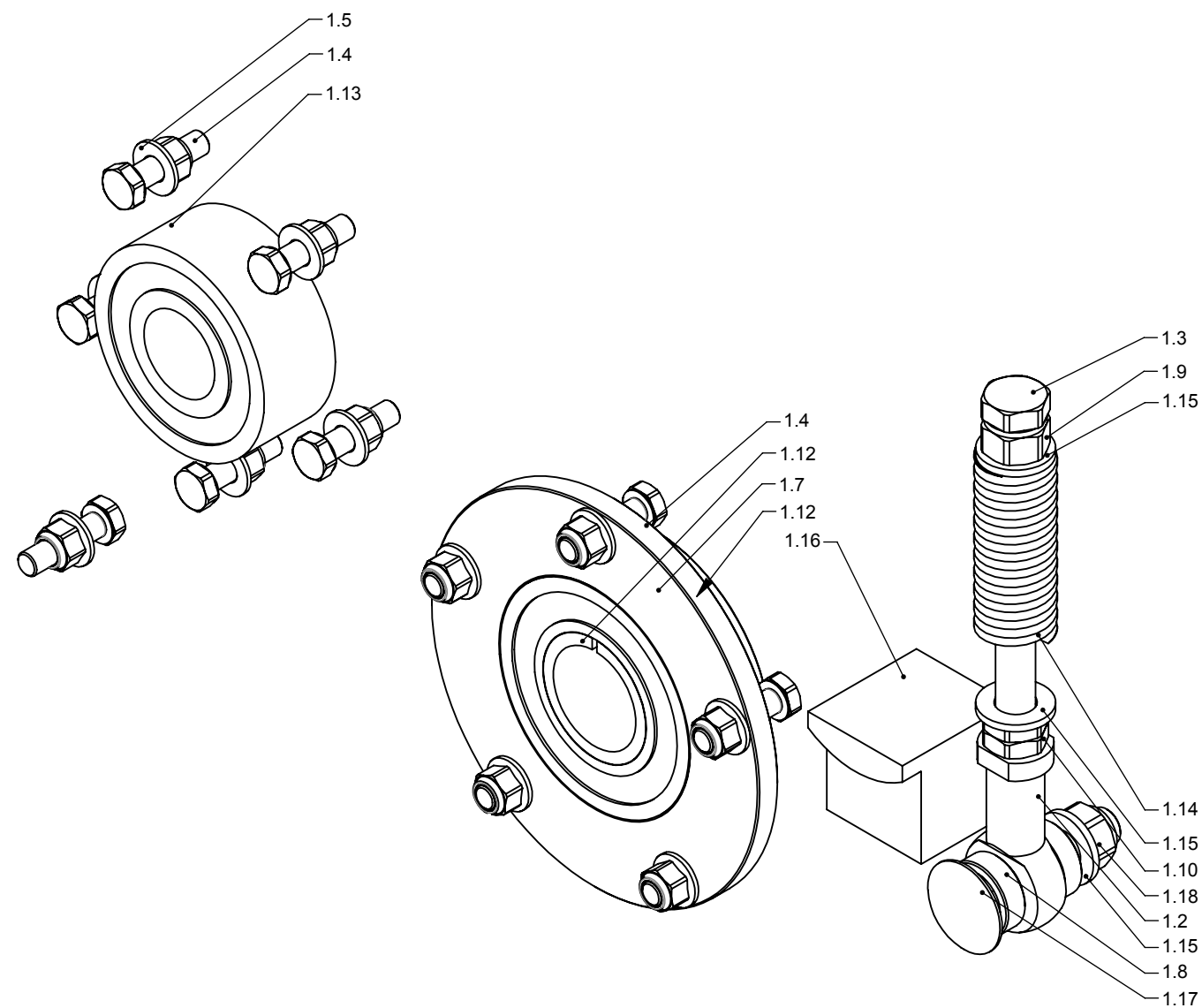
DETAIL A (1 : 2)
