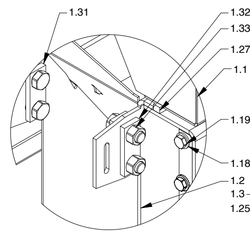
DETAIL F (1 : 5)
