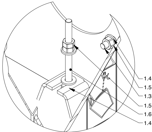
DETAIL B (1 : 3)
