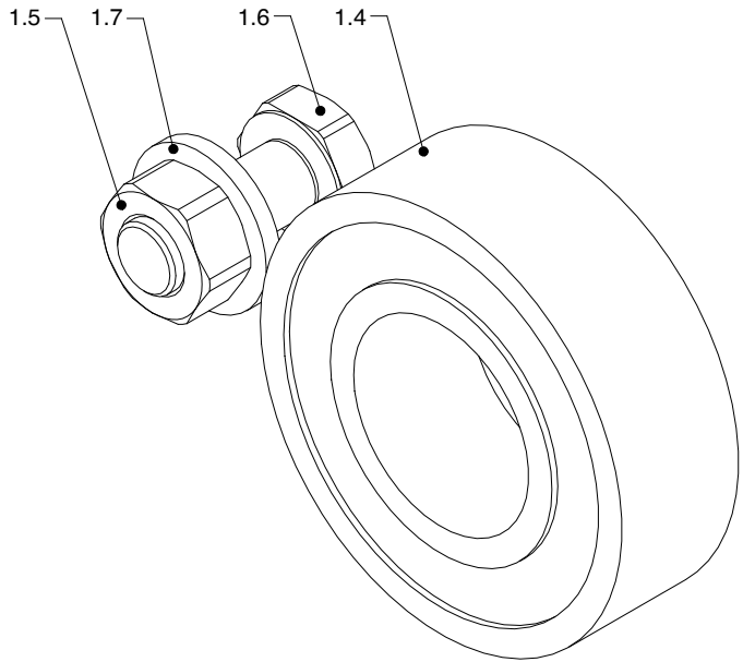
DETAIL A (1 : 1)
