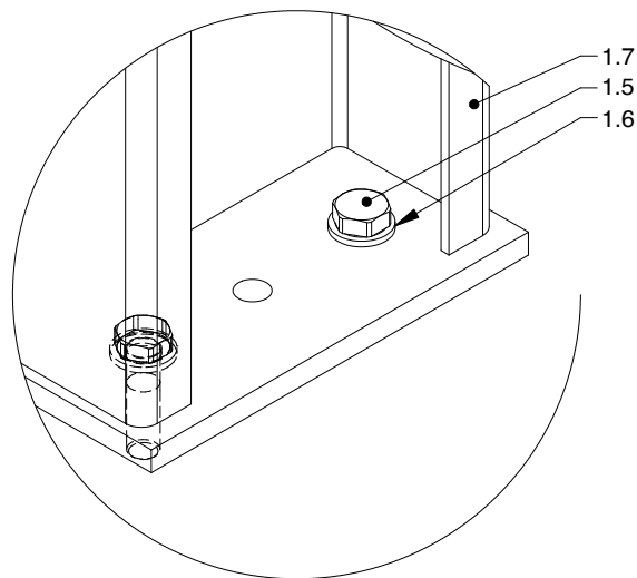
DETAIL B (1 : 3)
