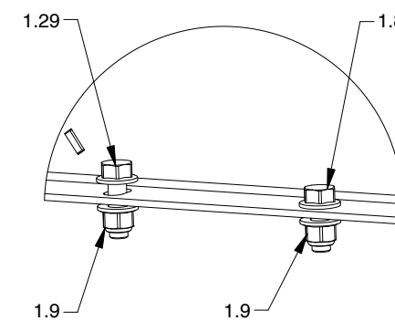
DETAIL G (1 : 3)
