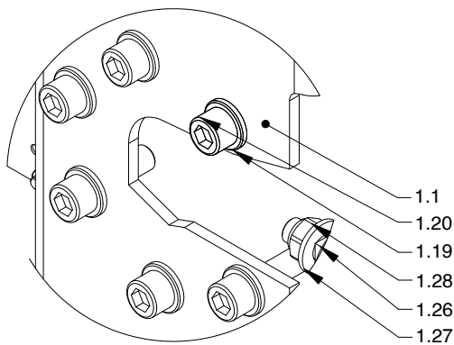
DETAIL C (1 : 3)
