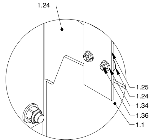
DETAIL E (1 : 3)
