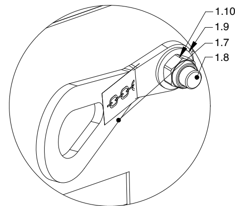
DETAIL G (1 : 3)
