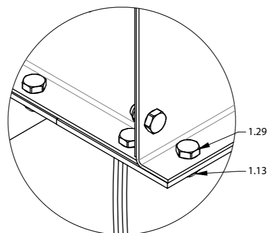
DETAIL C (1 : 3)
