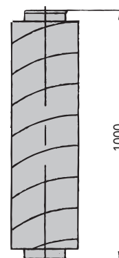
Silencer, galv. 125 500 552
