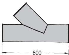
45° branch pipe, grey. OK160/100/160. 122 000 323
