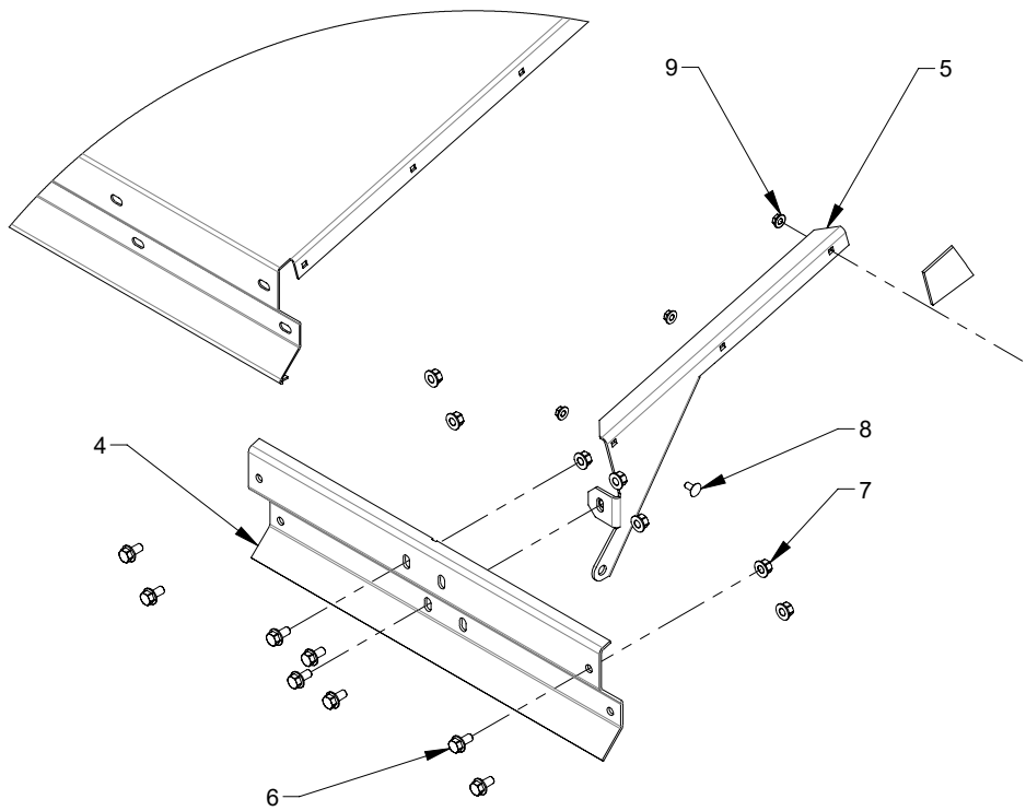
DETAIL A
