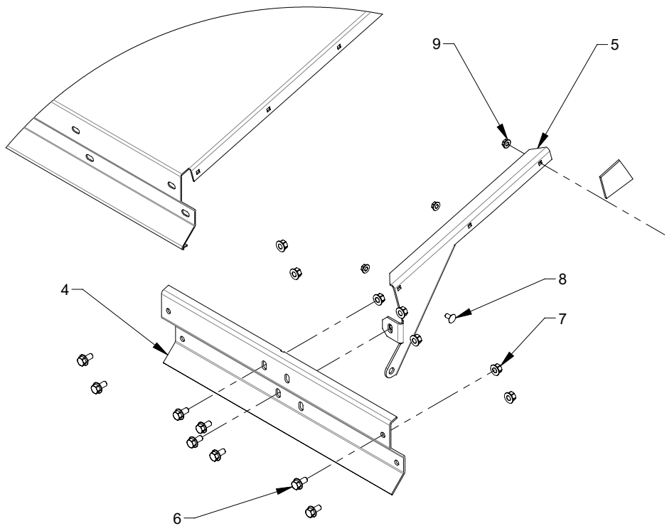
DETAIL A
