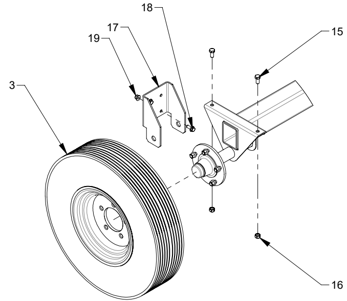
DETAIL C
