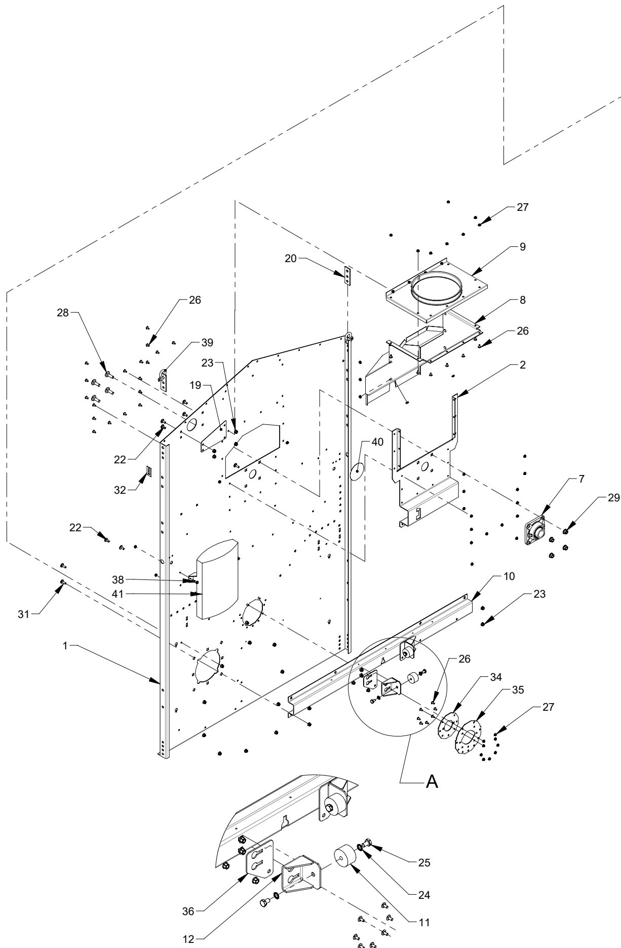
DETAIL A
