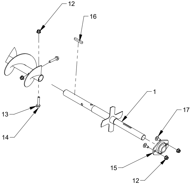
DETAIL B
