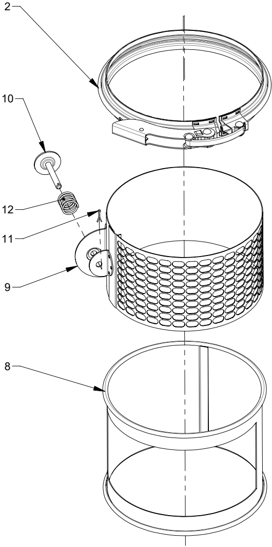
DETAIL A
