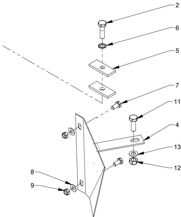
DETAIL A
