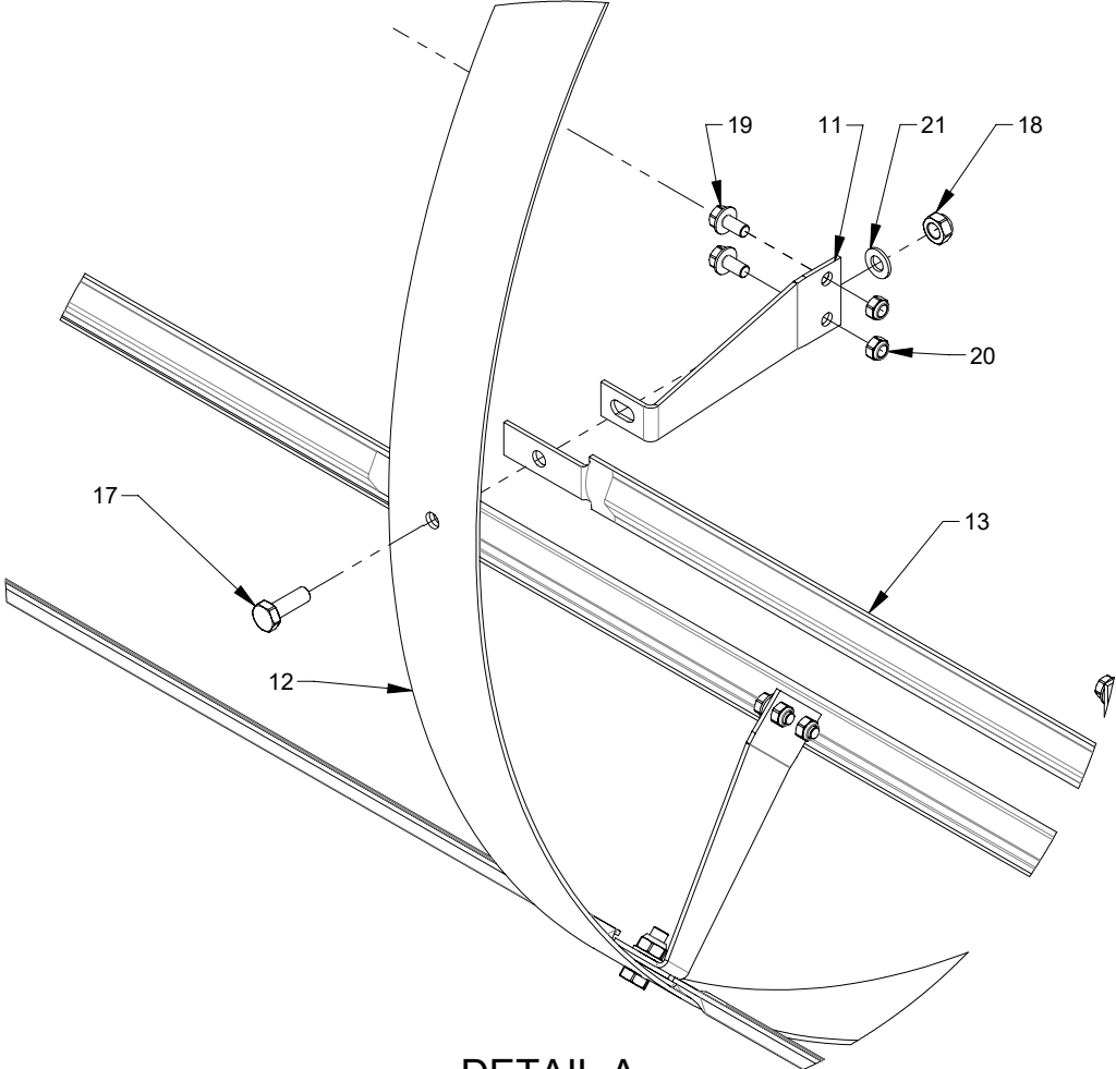
DETAIL A
