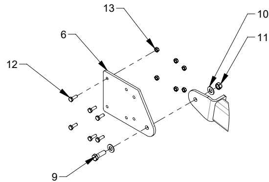
DETAIL B
