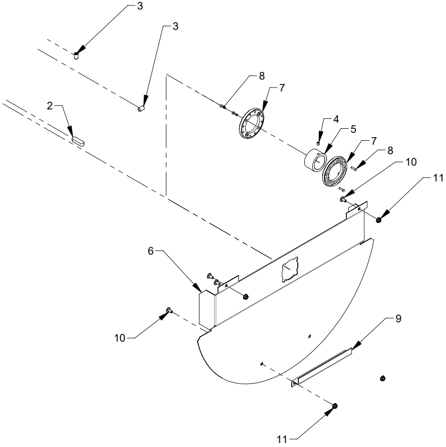
DETAIL A
