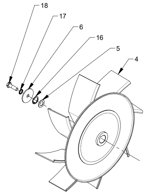
DETAIL B
