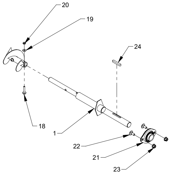
DETAIL B
