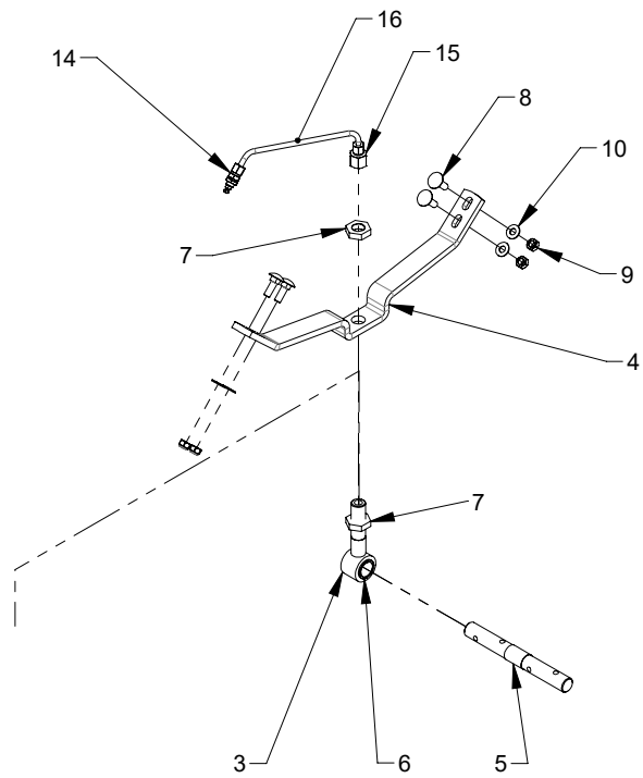
DETAIL A
