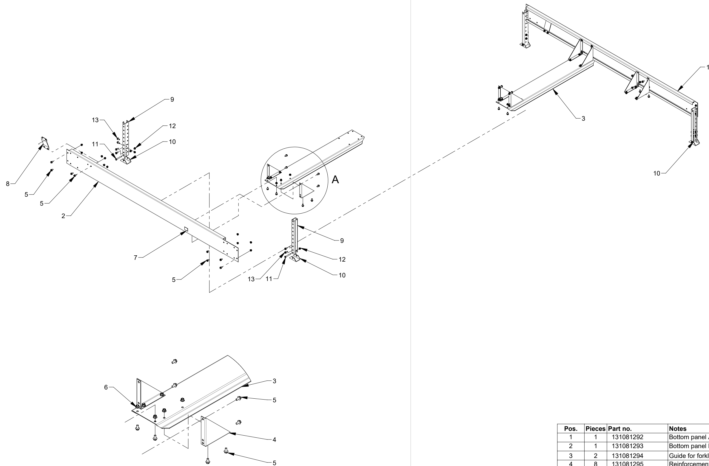
DETAIL A
