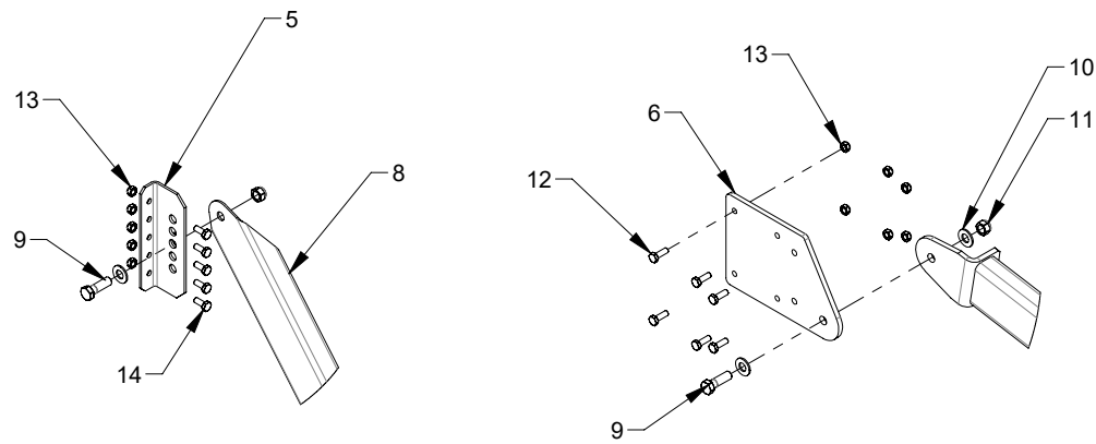
DETAIL A
