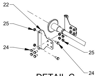
DETAIL C
