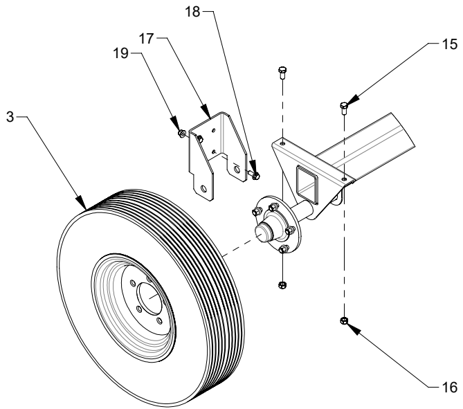
DETAIL C
