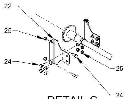
DETAIL C
