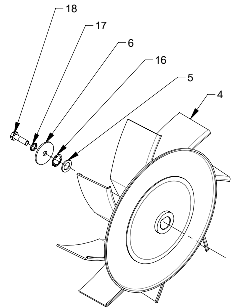
DETAIL B
