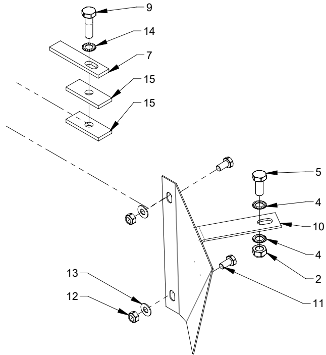
DETAIL A
