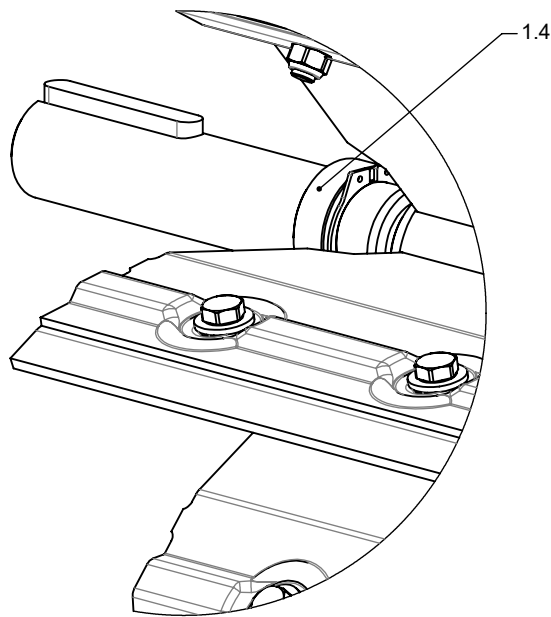
DETAIL C (2 : 5)
