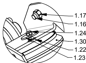
DETAIL G (1 : 5)
