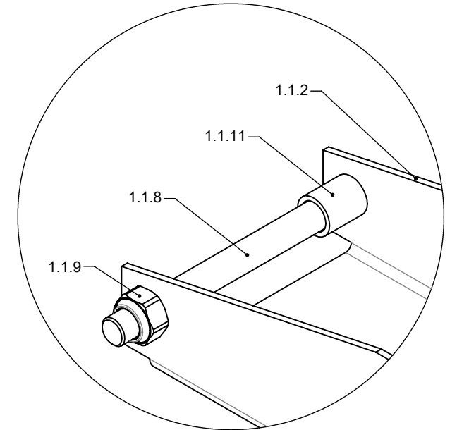
DETAIL C (1 : 2)
