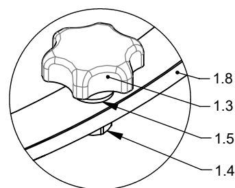
DETAIL A (1 : 2)
