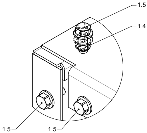
DETAIL C (1 : 2)
