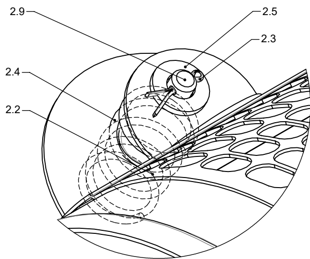
DETAIL B (1 : 1)
