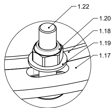
DETAIL B (1 : 1)
