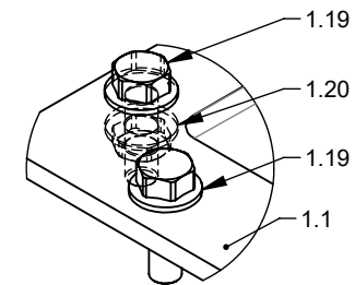
DETAIL F (1 : 2)
