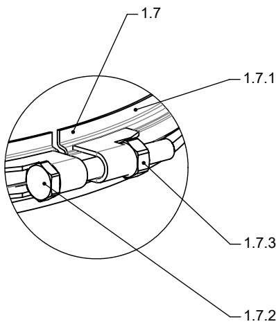
DETAIL A (2 : 5)
