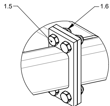
DETAIL A (1 : 5)
