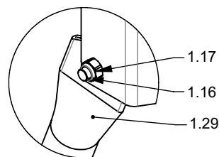
DETAIL H (1 : 5)
