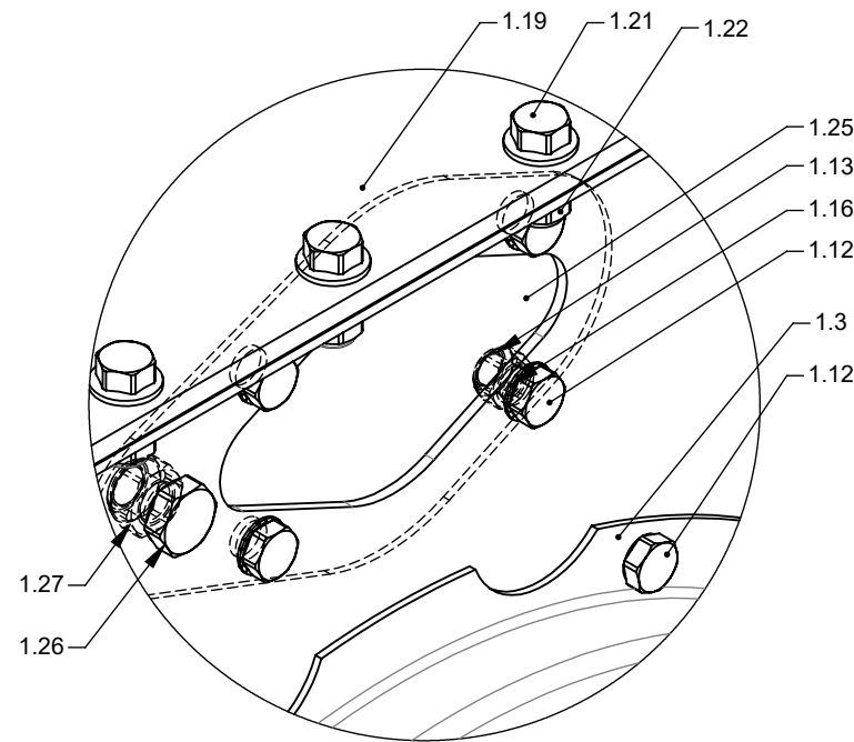
DETAIL A (1 : 2)
