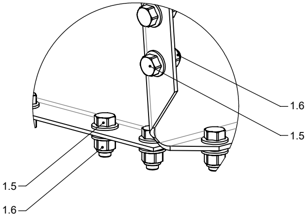
DETAIL B (2 : 5)
