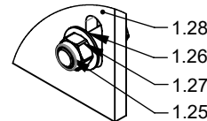
DETAIL E (1 : 5)
