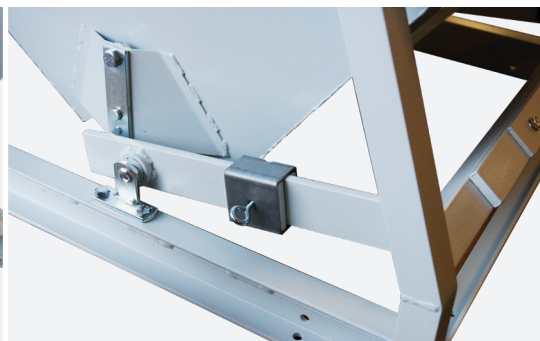
KA batch weigher adjustment.
