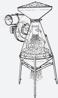
KF 12 mode of operation.
