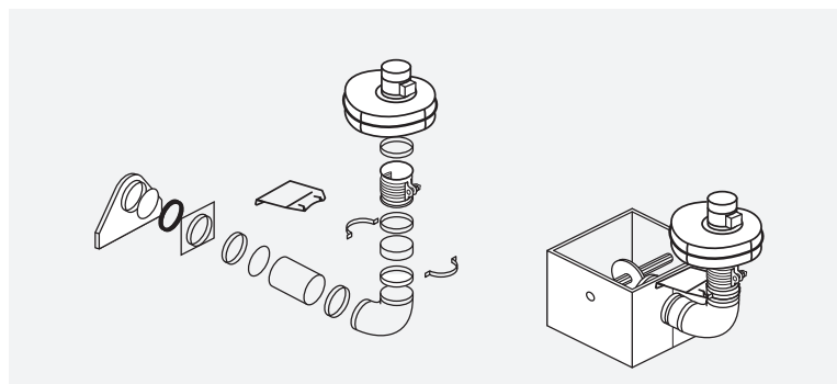
Super B Conveyor Mount
