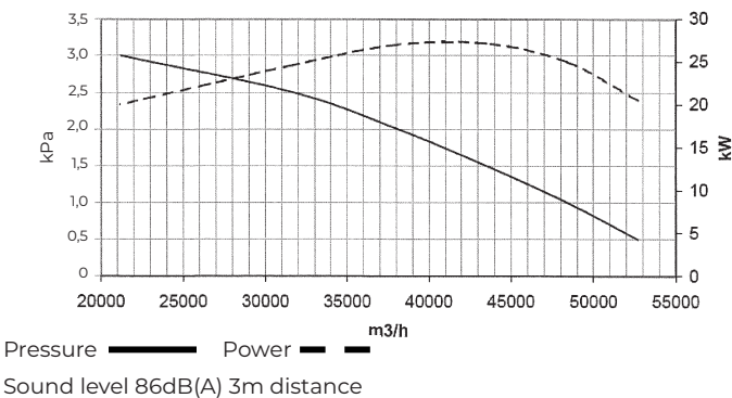
Air Volume for HVL400G (all positions)
