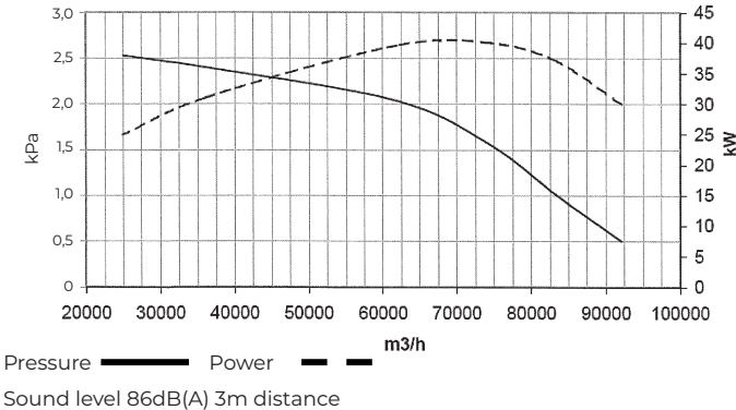
Air Volume for HVL600G (all positions)
