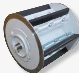
Rotor for CA 20 rotary valve fitted with rubber paddles.
